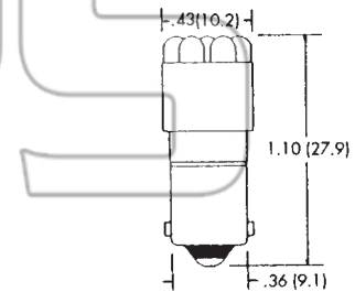
Fig. 2. Lamp with Bayonet Base
