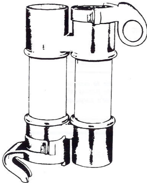
Fig. 2 Size DD Fuse Unit Assembled with Fittings for Type EK-3DD Fuse Disconnecting Switch
