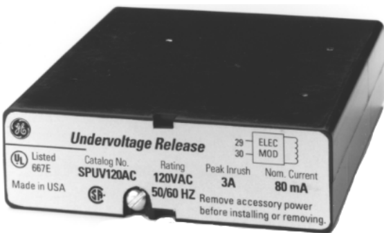
Figure 1. Undervoltage Release.
