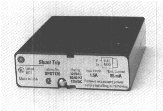
Figure 1. Shunt Trip.
