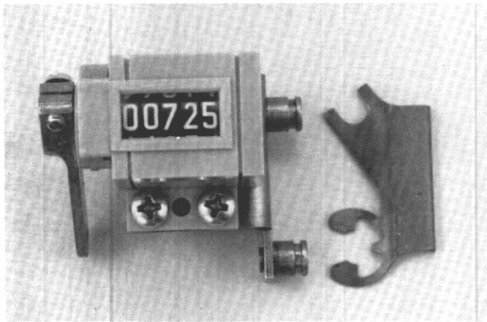
Figure 1. Mechanical Counter.
