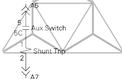
Figure 6. Shunt Trip connections to the secondary disconnect.
