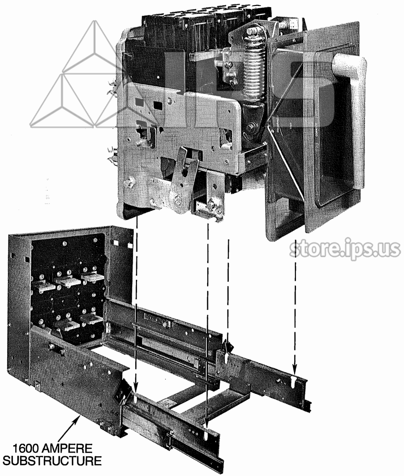
Figure 4. AKR-50 breaker, B-type drawout substructure mounting, manually operated
