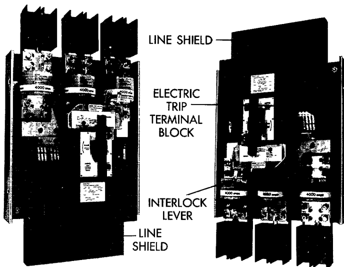
BOTTOM FEED
