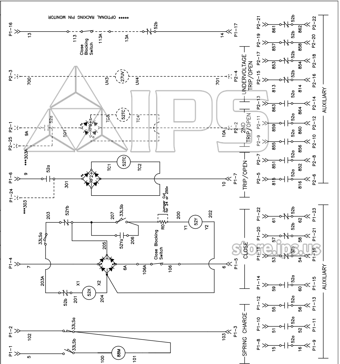
(N10) OPTIONAL ADVAC EU. SCHEMATIC W.D. Breaker shown in OPEN & CHARGED condition
